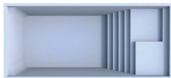
BETHA 12'x24' Depth: 4'11"
